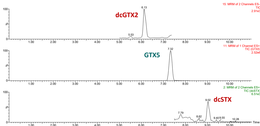
Figure 1. Analysis of the CRM-00-GTX5 (22-001) by UPLC-MS/MS. Conditions: ACQUITY UPLC Glycan BEH AMIDE 1.7 \mu m, (150 x 2.1) mm, UPLC column. Elution conditions, gradient mode with mobile phases: (A) [FmONH 4 ] = 1.0 mM and (B) acetonitrile/water 95/5 v/v with 0.01% FmOH; Gradient: 0 min 73% B; 5.0 min 73% B; 7.5 min 40% B; 7.6 min 20% B; 9.5 min 20% B; 9.6 min 73% B; 11.0 min 73% B; flow rate: 0.40 mL/min. Temperature: 55°C. MS detector: Waters XEVO TQ MS using the typical MRM transitions for PSPs analogues. TIC with the most important transitions for the main components and impurities are shown.
