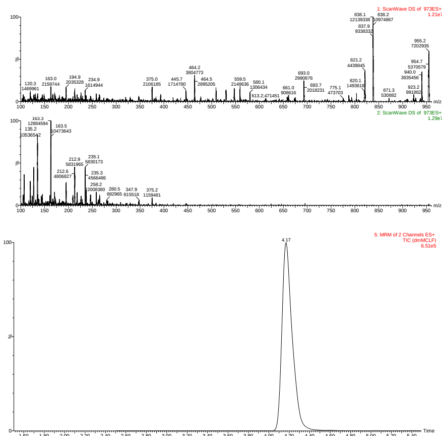
Figure 1. Analysis of the [D-Asp 3 ] microcystin-LF by UPLC-MS/MS. Conditions: ACQUITY UPLC HSS T3 1.7µm, 100x2.1 mm, UPLC column. Main elution conditions, gradient mode with mobile phases: (A) Water and (B) acetonitrile, both with 0.1% formic acid; Gradient: 0 min 30% B; 0.8 min 30% B; 2.5 min 60% B; 5.0 min 100% B; 5.5 min 100% B; 5.6 min 30% B; flow rate: 0.3 mL/min. Temperature: 30°C. The MS analysis includes MRM transitions of the most relevant Microcystins and main expected impurities. Superimposed spectrum: [D-Asp 3 ] microcystin-LF fragmentation pattern.
