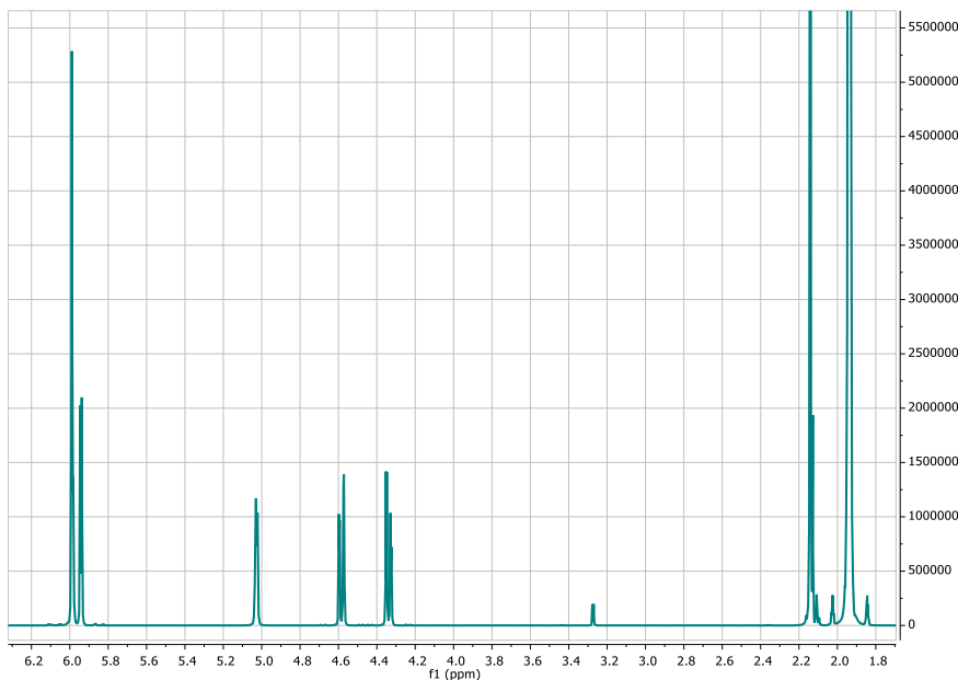
Figure 1. ^1\text{H} -NMR spectrum of Patulin solution, NEO AVANCE 750, 25mM of PAT in \text{CD}_3\text{CN} used in preparation of CRM-03-PAT batch 25-001. No identified impurities are highlighted.
