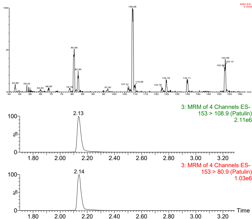
Figure 2. Analysis of the CRM-03-PAT (25-001) by UPLC-MS/MS. Conditions: ACQUITY UPLC HSS T3 1.7 \mu\text{m} , 100x2.1 mm, UPLC column. Mobile phases: (A) water containing 0.05% (v/v) acetic acid and 5 mM ammonium acetate, and (B) methanol. Gradient program: 0.00 min, 1% B; 1.00 min, 1% B; 2.00 min, 90% B; 2.50 min, 90% B; 3.50 min, 1% B; 5.50 min, 1% B. Flow rate: 0.5 mL/min. Column temperature: 40 ^\circ\text{C} . The scan spectrum is shown in the upper part of the figure.
