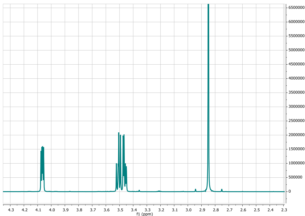
Figure 1. ^1\text{H} -NMR spectrum of L-BMAA·HCl solution, NEO AVANCE 750, 25mM of L-BMAA·HCl in \text{D}_2\text{O} used in preparation of CRM-03-BMAA batch 25-001.
