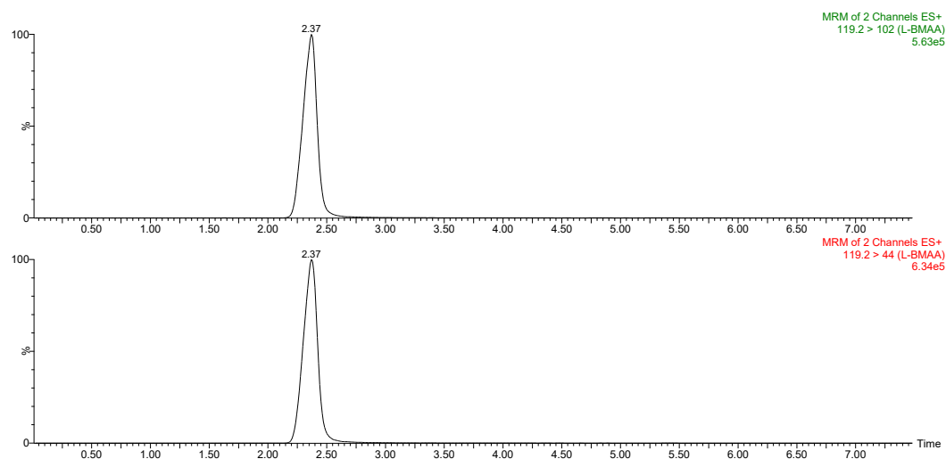
Figure 2. Analysis of the CRM-03-BMAA (25-001) solution by UPLC-MS/MS. Conditions: ACQUITY UPLC BEH AMIDE 1.7 \mu\text{m} , (150 x 2.1) mm, UPLC column. Elution conditions, gradient mode with mobile phases: (A) Water (0.1% FmOH), (B) Acetonitrile (0.1% FmOH); Gradient: 0 min 70% B; 4.0 min 70% B; 4.5 min 40% B; 5.9 min 40% B; 6.0 min 70% B; 7.5 min 70% B; flow rate: 0.40 mL/min. Temperature: 55°C. MS detector: Waters XEVO TQ MS.
