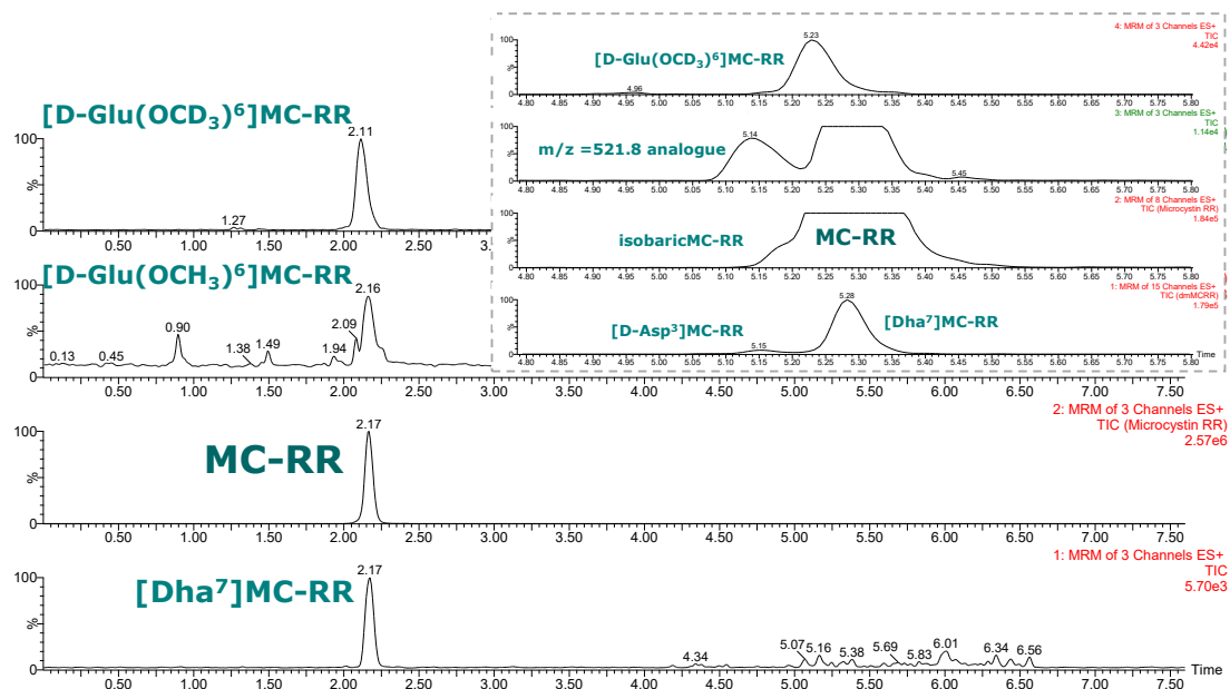
Figure 1. Analysis of the CRM-00-MCRR (23-001) by UPLC-MS/MS. Conditions: ACQUITY UPLC HSS T3 1.7 \mu m, 100x2.1 mm, UPLC column. Main elution conditions, gradient mode with mobile phases: (A) Water and (B) acetonitrile, both with 0.1% formic acid; Gradient: 0 min 30% B; 0.8 min 30% B; 2.5 min 60% B; 5.0 min 100% B; 5.5 min 100% B; 5.6 min 30% B; flow rate: 0.3 mL/min. Temperature: 30°C. MS detector: Waters XEVO TQ-MS using the typical MRM transitions of the most relevant Microcystins and main expected impurities. Superimposed chromatogram, gradient modified to enhanced selectivity, highlights other minor analogues as impurities.
