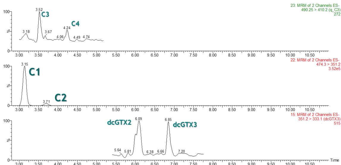
Figure 1. Analysis of the CRM-00-C1&2 solution by HPLC-MS/MS. Conditions: ACQUITY UPLC BEH AMIDE 1.7µm, (150 x 2.1) mm, UPLC column. Elution conditions, gradient mode with mobile phases: (A) [FmONH 4 ] = 1.0 mM (B) Aqueous 95% acetonitrile with 0.01% FmOH; Gradient: 0 min 73% B; 5.0 min 73% B; 7.5 min 40% B; 7.6 min 20% B; 9.5 min 20% B; 9.6 min 73% B; 11.0 min 73% B; flow rate: 0.40 mL/min. Temperature: 55°C. MS detector: Waters XEVO TQ MS using the typical MRM transitions for PSPs analogues.
