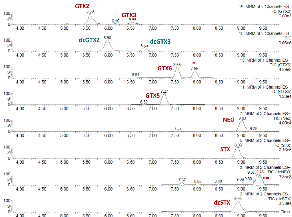
Figure 1. Analysis of the CRM-00-dcGTX2&3 (22-001) by UPLC-MS/MS. Conditions: ACQUITY UPLC BEH AMIDE 1.7µm, (100 x 2.1) mm, UPLC column. Elution conditions, gradient mode with mobile phases: (A) [FmONH 4 ] = 1.0 mM (B) Aqueous 95% acetonitrile with 0.01% FmOH; Gradient: 0 min 73% B; 5.0 min 73% B; 7.5 min 40% B; 7.6 min 20% B; 9.5 min 20% B; 9.6 min 73% B; 11.0 min 73% B; flow rate: 0.40 mL/min. Temperature: 55°C. MS detector: Waters XEVO TQ MS using the typical MRM transitions for PSPs analogues. TIC with the most important transitions for the main components and impurities are shown. (*) Unknown impurity with 396.2 > 316.1 MRM transition. (**) Unknown impurity with the same transitions as dcNEO.
