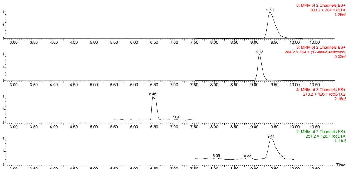
Figure 1. Analysis of the CRM-00-STX (24-001) by UPLC-MS/MS. Conditions: ACQUITY UPLC Glycan BEH AMIDE 1.7 \mu m, (150 x 2.1) mm, UPLC column. Elution conditions, gradient mode with mobile phases: (A) [FmONH 4 ] = 1.0 mM (B) acetonitrile/water 95/5 v/v with 0.01% FmOH; Gradient: 0 min 73% B; 5.0 min 73% B; 7.5 min 40% B; 7.6 min 20% B; 9.5 min 20% B; 9.6 min 73% B; 11.0 min 73% B; flow rate: 0.40 mL/min. Temperature: 55°C. MS detector: Waters XEVO TQ MS using the typical MRM transitions for PSPS analogues.
