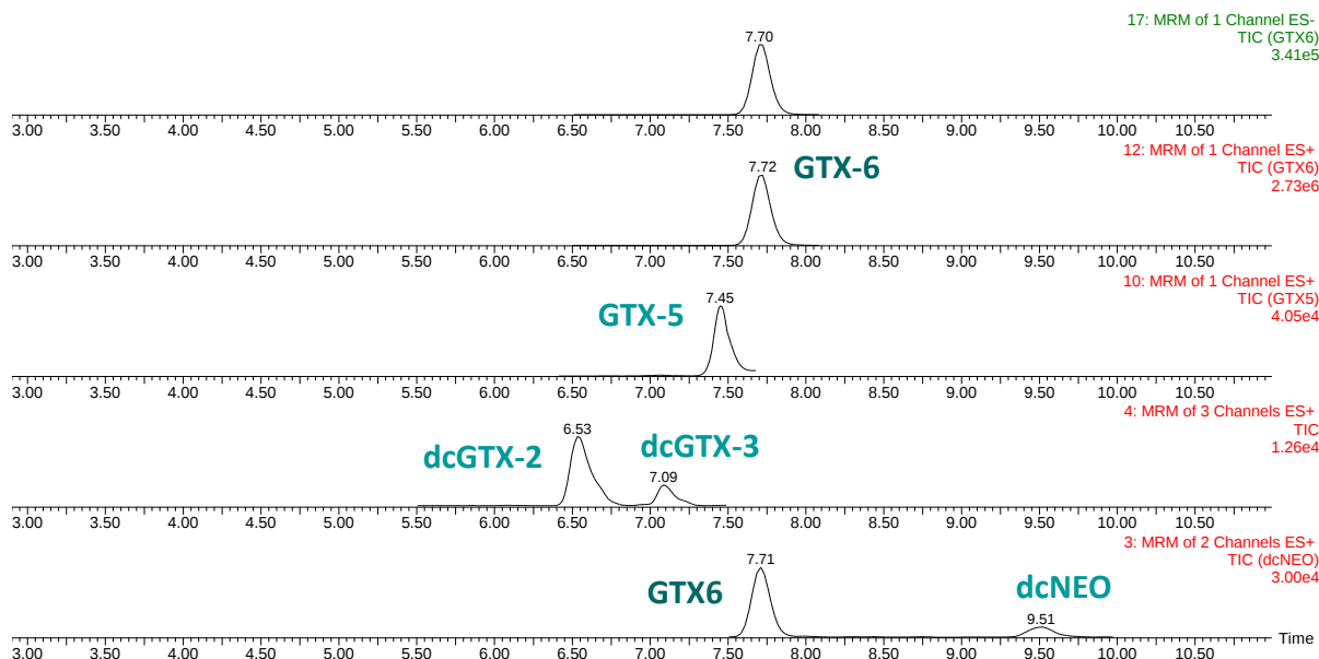
Figure 1. Analysis of the CRM-00-GTX6 solution by HPLC-MS/MS. Conditions: ACQUITY UPLC BEH AMIDE 1.7 \mu m, (150 x 2.1) mm, UPLC column. Elution conditions, gradient mode with mobile phases: (A) [FmONH 4 ] = 1.0 mM (B) Aqueous 95% acetonitrile with 0.01% FmOH; Gradient: 0 min 73% B; 5.0 min 73% B; 7.5 min 40% B; 7.6 min 20% B; 9.5 min 20% B; 9.6 min 73% B; 11.0 min 73% B; flow rate: 0.40 mL/min. Temperature: 55°C. MS detector: Waters XEVO TQ MS using the typical MRM transitions for PSPs analogues.
