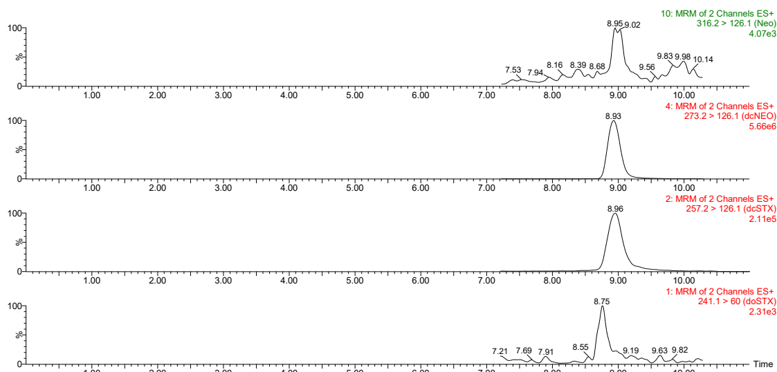
Figure 1. Analysis of the CRM-00-dcNEO (23-001) by UPLC-MS/MS. Conditions: ACQUITY UPLC Glycan BEH AMIDE 1.7 \mu m, (150 x 2.1) mm, UPLC column. Elution conditions, gradient mode with mobile phases: (A) [FmONH 4 ] = 1.0 mM and (B) acetonitrile/water 95/5 v/v with 0.01% FmOH; Gradient: 0 min 73% B; 5.0 min 73% B; 7.5 min 40% B; 7.6 min 20% B; 9.5 min 20% B; 9.6 min 73% B; 11.0 min 73% B; flow rate: 0.40 mL/min. Temperature: 55 °C. MS detector: Waters XEVO TQ MS using the typical MRM transitions for PSPs analogues. TIC with the most important transitions for the main component and impurities are shown.
