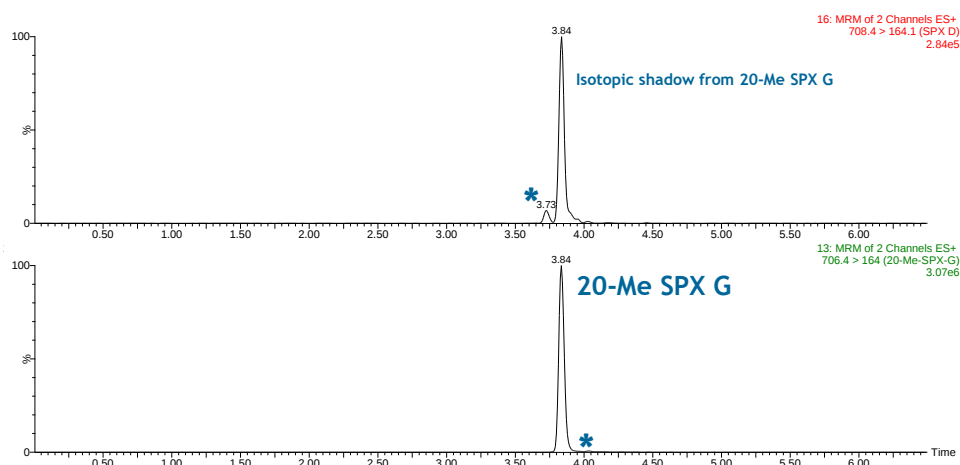
Figure 1. Analysis of the 20-methyl Spirolide G by UPLC-MS/MS. Conditions: ACQUITY UPLC BEH C18 1.7 \mu m, 100x2.1 mm, UPLC column. Elution conditions, gradient mode with mobile phases: (A) Water and (B) Aqueous 95% acetonitrile, both with 2mM ammonium formate and 50mM formic acid; Gradient: 0 min 10% B; 4.5 min 65% B; 5.5 min 65% B; 5.6 min 10% B; 6.5 min 10% B; flow rate: 0.4 mL/min. Temperature: 30°C. MS detector: Waters XEVO TQ MS using the typical MRM transitions of spirolide toxin group found in the bibliography. Detected impurities are highlighted.
