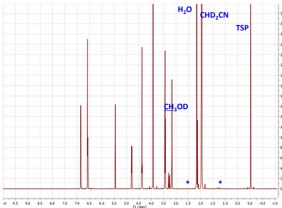
Figure 1. ^1\text{H} -NMR spectrum of AFG1 solution, Varian 500 MHz, 15mM of AFG1 in \text{CD}_3\text{CN} used in preparation of CRM-03-AFG1 batch 17-001. No identified impurities are highlighted. As the structure of these impurities is not known, their exact amount cannot be calculated. Because the impurities usually are smaller molecules (otherwise, more NMR signals would arise), it can be estimated from the corresponding integrals, but this purity is not relative to close-related impurities to Aflatoxin G1 analogues.
