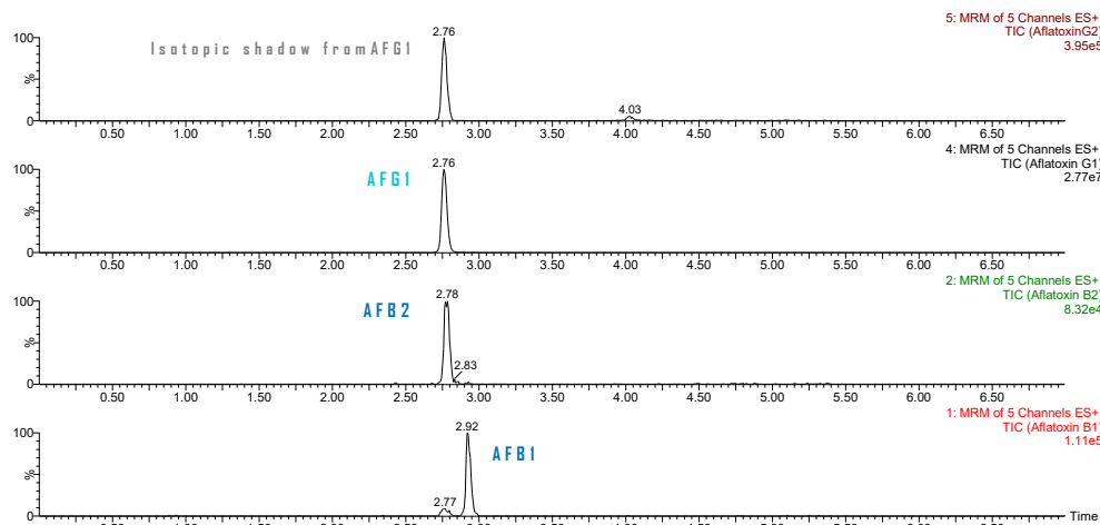
Figure 2. Analysis of the CRM-03-AFG1 (17-001) by UPLC-MS/MS. Conditions: ACQUITY UPLC HSS T3 1.7 \mu\text{m} , 100x2.1 mm, UPLC column. Elution conditions, gradient mode with mobile phases: (A) Water and (B) Acetonitrile, both with 0.1% formic acid (v/v); Gradient: 0 min 25% B; 0.60 min 25% B; 4.35 min 100% B; 5.60 min 100% B; 6.00 min 25% B; 7.00 min 25% B; flow rate: 0.3 mL/min. Temperature: 40 °C. MS detector: Waters XEVO TQ-MS using 4 MRM transitions for each Aflatoxin derivative.
