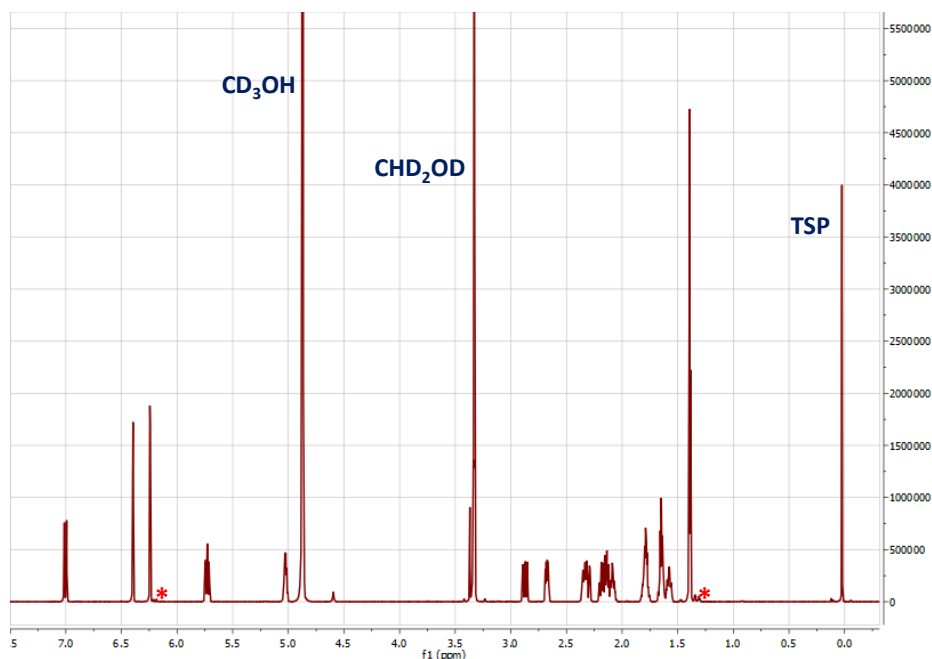
Figure 1. ^1\text{H} -NMR spectrum of Zearalenone solution, Bruker NEO 750, 16 mM of ZON in \text{CD}_3\text{OD} used in preparation of CRM-00-ZON batch 19-001. No identified impurities are highlighted. As the structure of these impurities is not known, their exact amount cannot be calculated. Because the impurities usually are smaller molecules (otherwise, more NMR signals would arise), it can be estimated from the corresponding integrals, but this purity is not relative to close-related impurities to Zearalenone analogues.
