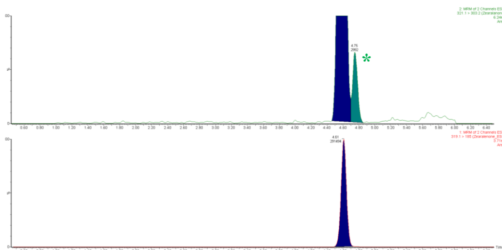
Figure 2. Analysis of the CRM-00-ZON (19-001) by UPLC-MS/MS. Conditions: ACQUITY UPLC HSS T3 1.7 \mu\text{m} , 100x2.1 mm, UPLC column. Elution conditions, gradient mode with mobile phases: (A) Water and (B) acetonitrile, both with 0.1% formic acid; Gradient: 0 min 15% B; 0.8 min 15% B; 4.3 min 70% B; 4.4 min 90% B; 5.4 min 90% B; 5.5 min 15% B; flow rate: 0.4 mL/min. Temperature: 40°C. MS detector: Waters XEVO TQ-MS using MRM transitions of Zearalenone. (*) denotes a signal under Zearalenone MRM channel, unknown impurity.
