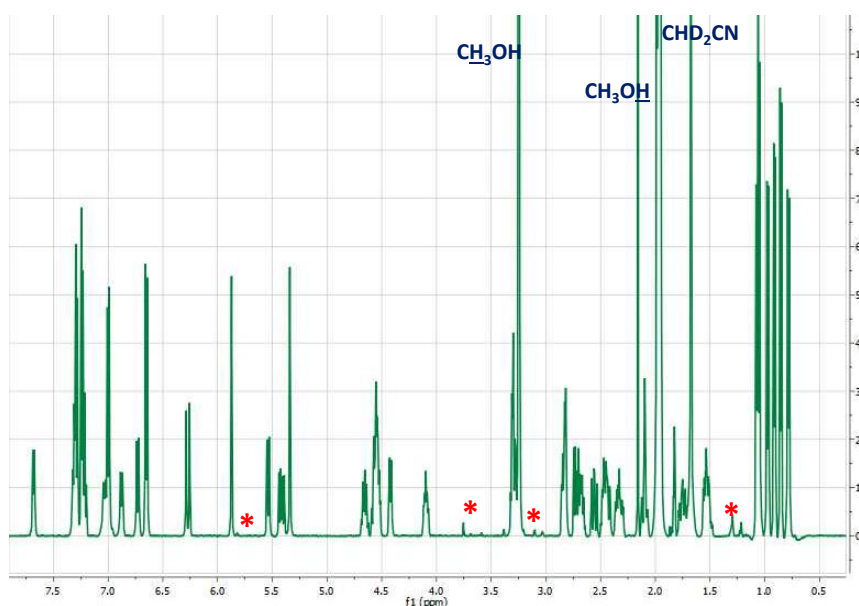
Figure 1. ^1\text{H} -NMR spectrum of MCLY solution, VARIAN 500 WB, 3 mM of MCLY in \text{CD}_3\text{CN} used in preparation of CRM-00-MCLY batch 19-001. No identified impurities are highlighted. As the structure of these impurities is not known, their exact amount cannot be calculated. Because the impurities usually are smaller molecules (otherwise, more NMR signals would arise), it can be estimated from the corresponding integrals, but this purity is not relative to close-related impurities to microcystin analogues.
