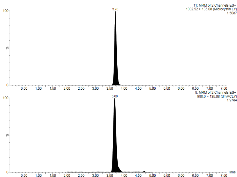
Figure 2. Analysis of the CRM-00-MCLY (19-001) by UPLC-MS/MS. Conditions: ACQUITY UPLC HSS T3 1.7 \mu\text{m} , 100x2.1 mm, UPLC column. Elution conditions, gradient mode with mobile phases: (A) Water and (B) acetonitrile, both with 0.1% formic acid; Gradient: 0 min 30% B; 0.8 min 30% B; 2.5 min 60% B; 5.0 min 100% B; 5.5 min 100% B; 5.6 min 30% B; 7.6 min 30% B; flow rate: 0.3 mL/min. Temperature: 30 °C. MS detector: Waters XEVO TQ-MS using the suitable MRM transition performance for each Microcystin.
