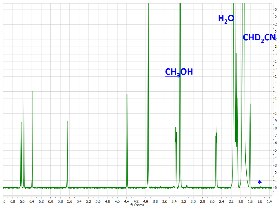
Figure 1. ^1\text{H} -NMR spectrum of AFM1 solution, Varian 500 MHz, 1.5mM of AFM1 in \text{CD}_3\text{CN} used in preparation of CRM-03-AFM1 batch 20-001. No identified impurities are highlighted. As the structure of these impurities is not known, their exact amount cannot be calculated. Because the impurities usually are smaller molecules (otherwise, more NMR signals would arise), it can be estimated from the corresponding integrals, but this purity is not relative to close-related impurities to Aflatoxin M1 analogues.
