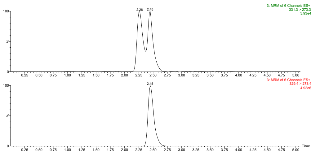
Figure 2. Analysis of the CRM-03-AFM1 (20-001) by UPLC-MS/MS. Conditions: ACQUITY UPLC HSS T3 1.7 \mu\text{m} , 100x2.1 mm, UPLC column. Elution conditions, gradient mode with mobile phases: (A) Water and (B) Acetonitrile, both with 0.1% formic acid (v/v); Gradient: 0 min 25% B; 0.60 min 25% B; 4.35 min 100% B; 5.60 min 100% B; 6.00 min 25% B; 7.00 min 25% B; flow rate: 0.3 mL/min. Temperature: 40°C. MS detector: Waters XEVO TQ-MS using typical MRM transitions for aflatoxins analogues. Tentative AFM2 analogue at 2.26 min is detected.
